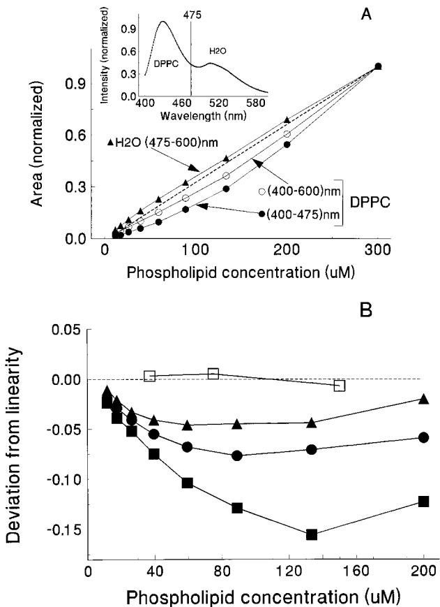
FIGURE 3 (A) Integrated emission intensity of Prodan as a function of the sample concentration in the buffer. Samples of 0.3 mM DPPC and 0.3 μM Prodan were progressively diluted by one-third with the buffer; the emission spectra were acquired at 25°C. On the y axis we report the integrated emission intensity of the total emission (from 400 nm to 600 nm; ○), of the emission attributed to the probe in DPPC (from 400 nm to 475 nm; ●), and of the emission attributed to the probe in water (from 475 nm to 600 nm; ▲), as shown in the inset. The straight dotted line is drawn for comparison. The deviation of the integrated emission from this last dotted line is reported in B, together with the deviation from linearity of the total integrated emission, from 400 nm to 550 nm, of a Laurdan-labeled DPPC sample, progressively diluted by one-half by a procedure similar to that used for the Prodan-labeled sample.
