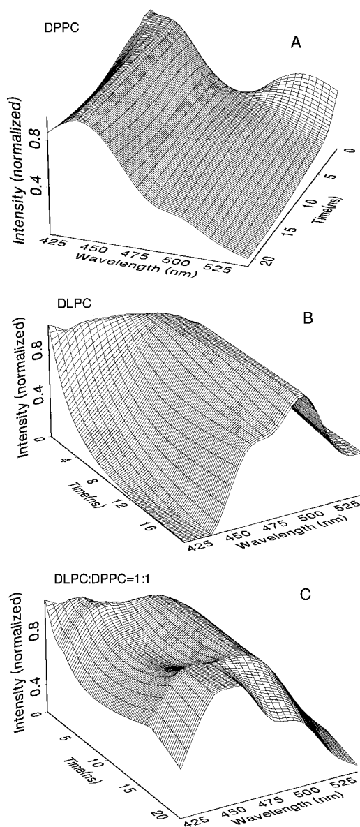
FIGURE 10 Prodan time-resolved emission spectra at 25°C in DPPC (A), DLPC (B), and DLPC:DPPC = 1:1 (C) multilamellar phospholipid vesicles.
